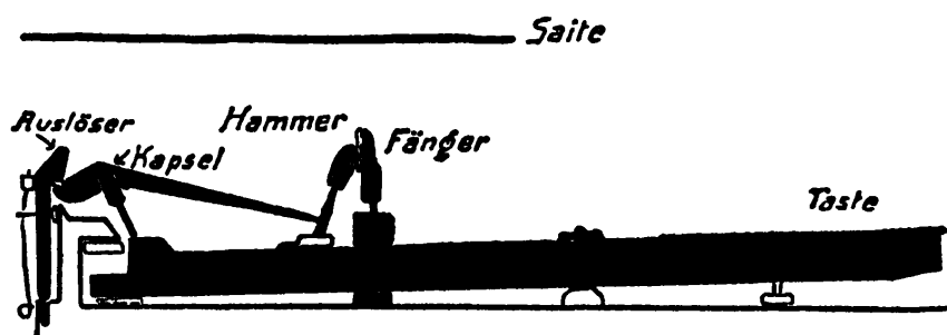
FIGURE 124. German Prellmechanik with escapement; del. Carmina Manger.
